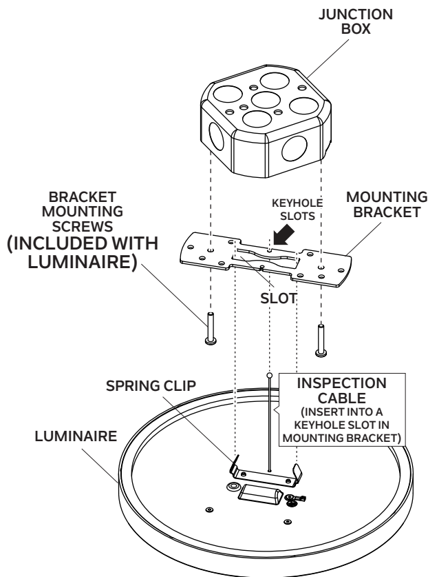
Fig. 1 INSTALLING TO STANDARD JUNCTION BOX
