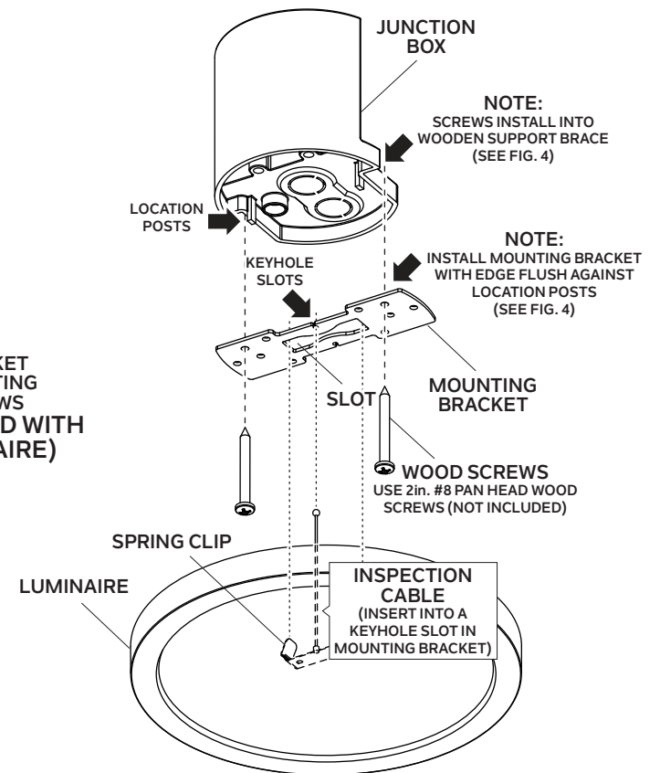
Fig. 3 INSTALLING TO L-SHAPED CEILING FAN JUNCTION BOX
